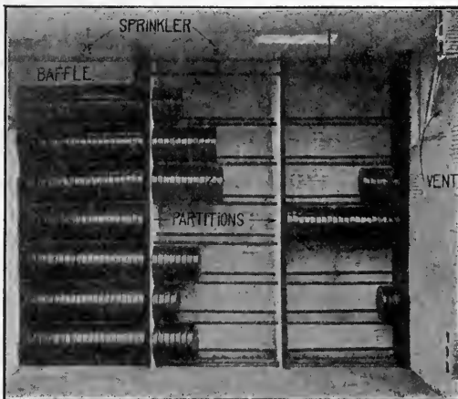
FIG. 3. Film storage vault. Showing construction of racks and installation of partitions, baffles, and sprinklers.
